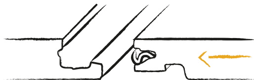
INSTALLATION METHOD 2 snap (horizontal)
